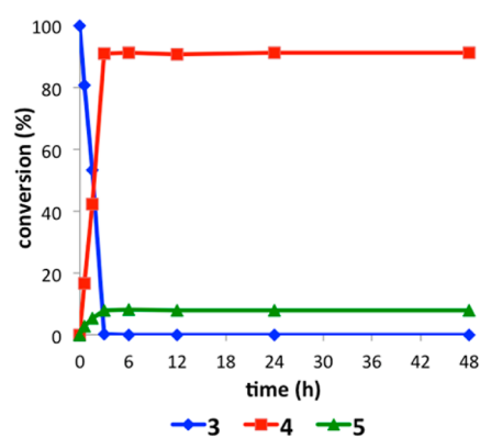
Figure 1. Reactions with MsOH (1.0 equiv). (a) Rate profile for catalyzed cyclization with 0.1 equiv of (S)-1. (b) Rate profile for uncatalyzed cyclization.
