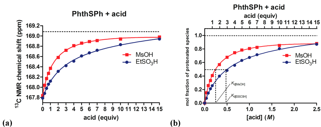
Figure 5. Titration curves for protonation of 2 with MsOH and EtSO 3 H.
